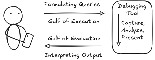
Figure 3: Programmers formulate their data needs as queries and interpret what the results mean about how the code executes. The types of expressible queries and the formats of the query and output are determined by the debugging tool being used.
