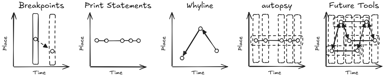
Figure 1: Analyzing debugging tools as mediums for foraging over place and time. We contribute a lens to support analysis of the expressive potential and efficiency of debugging tools. Programmers issue queries via their debugging tools to examine execution data across the axes of place (which encodes particular variables present at a source location) and time. Breakpoints capture variables at every level of the stack at a particular time. Print statements capture specific variables and the order that places are visited during execution. Whyline provides links between points in place-time according to cause and effect. Our transitional debugging tool autopsy blends views across place and aggregations across time. We envision that future debugging tools could combine these capabilities.
