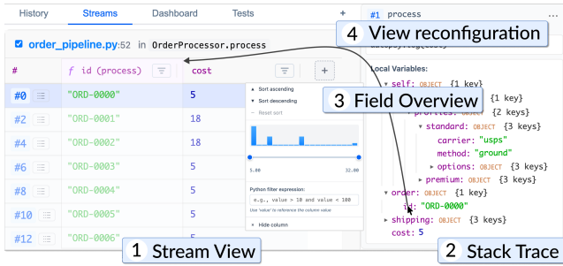
Figure 4: The autopsy interface. Captured logs are presented as tables in the Stream View (①). Clicking on any row shows the complete stack trace that was captured simultaneously with the log (②). Logged fields can have their distributions visualized, and can be used to filter and sort logs (③). Fields from the call stack can be added as columns to the table, enabling easier comparisons (④).
