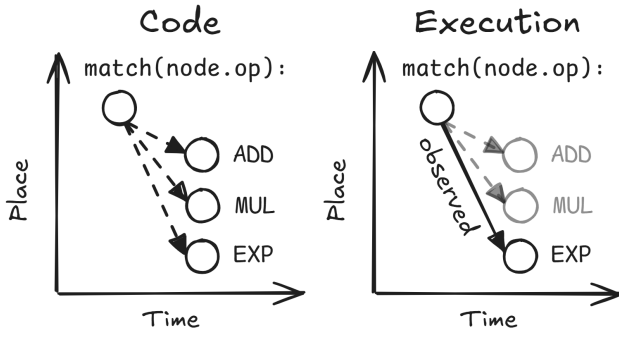
Figure 2: Querying execution data fulfills data needs. The student wonders which operator is evaluated first. Left: Control flow in code presents each operator case as a possible path of execution. Right: Interpreting the query result makes it clear that the exponentiation operator is evaluated first.
